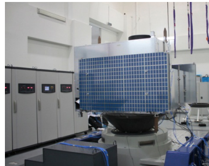
Fig.2 Mechanical environmental simulation test
