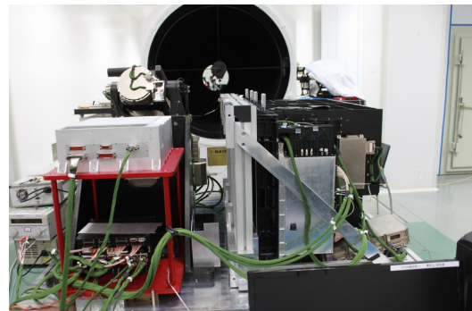
Fig.3 Joint test of satellite payload entanglement source
